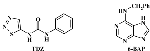
Scheme 2. The structure of phytohormones thiazuron (TDZ) and 6-benzylaminopurine (6-BAP).
