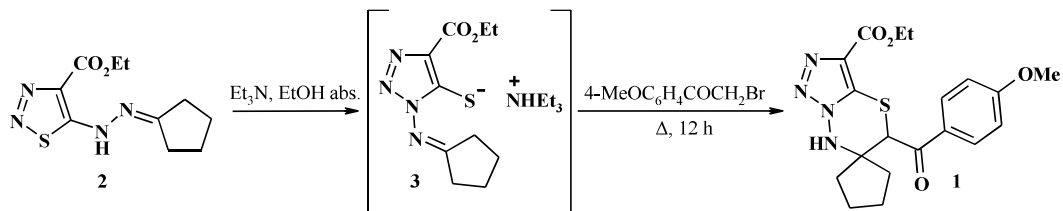
Scheme 1. Synthesis of STT.
