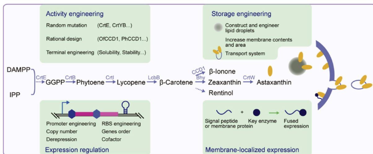
Fig. (2). Strategies for engineering the carotenoid biosynthesis module (Cheng et al. ) [52]. Open Access under a Creative Commons CC-BY-NC-ND license. No changes or alterations were made in the figure. https://www.sciencedirect.com/science/article/pii/S221403011930046X#fig3 . (A higher resolution / colour version of this figure is available in the electronic copy of the article).
