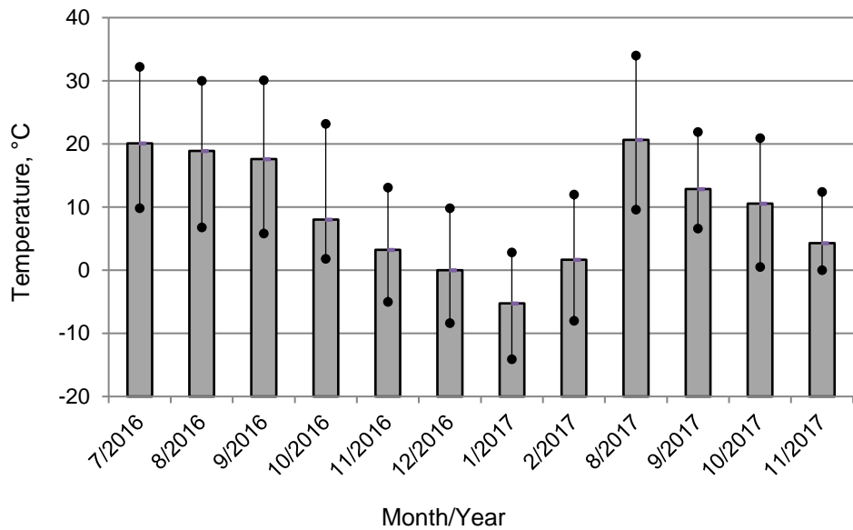
Figure 3. Monthly outside temperatures in the location of the observed storage facility.
